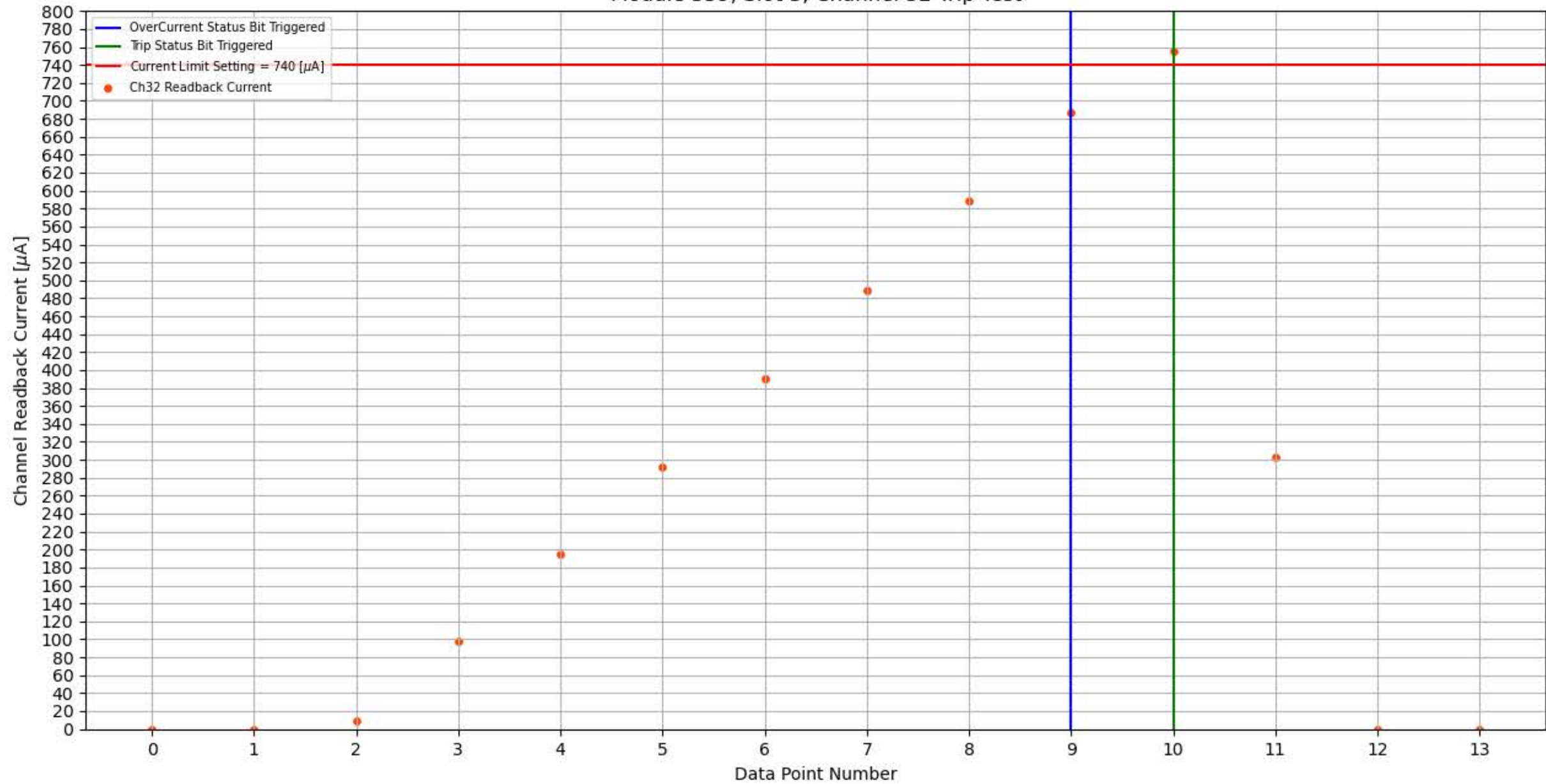
Module 359, Slot 3, Channel 32 Trip Test
