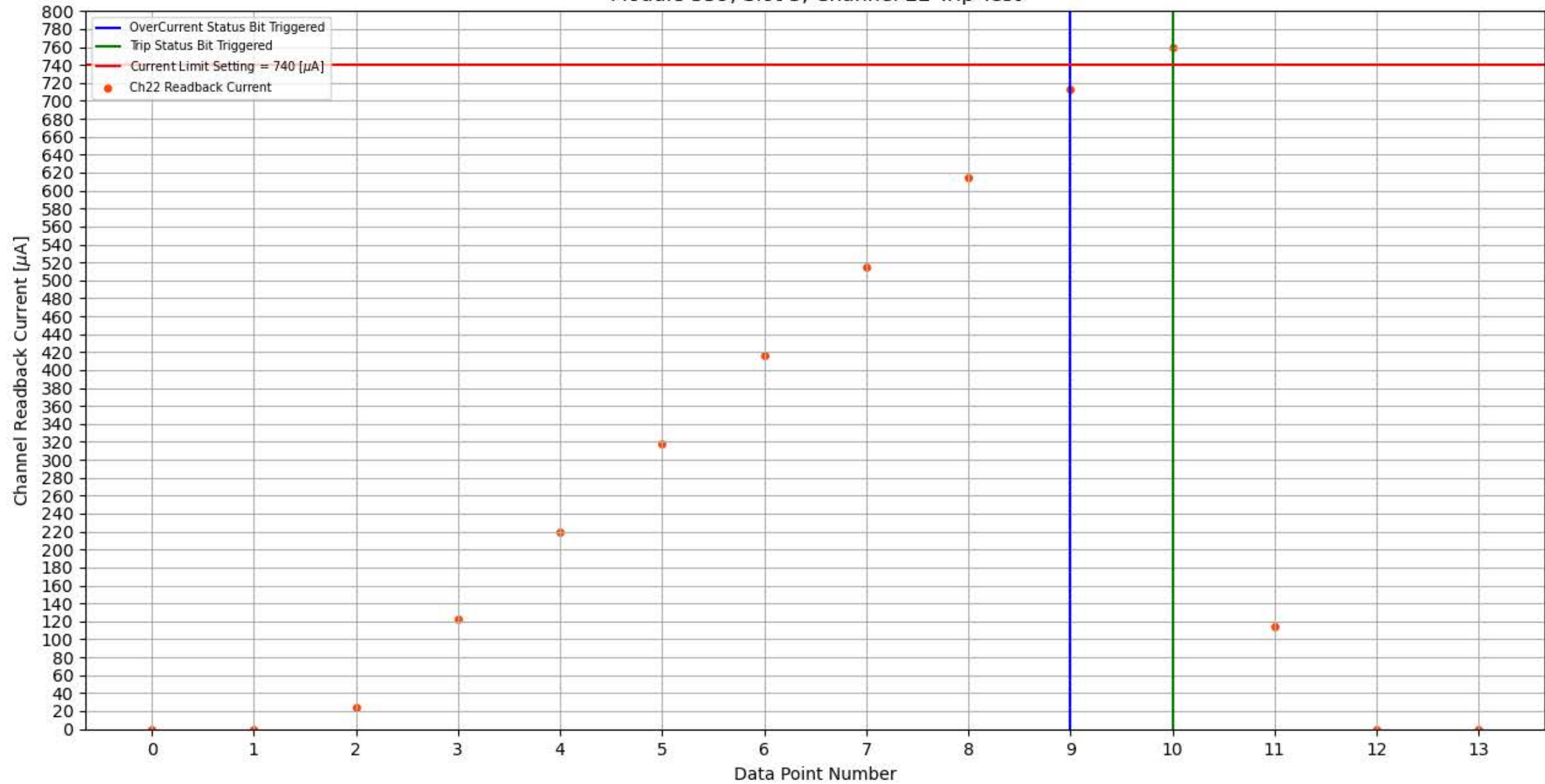
Module 359, Slot 3, Channel 22 Trip Test
