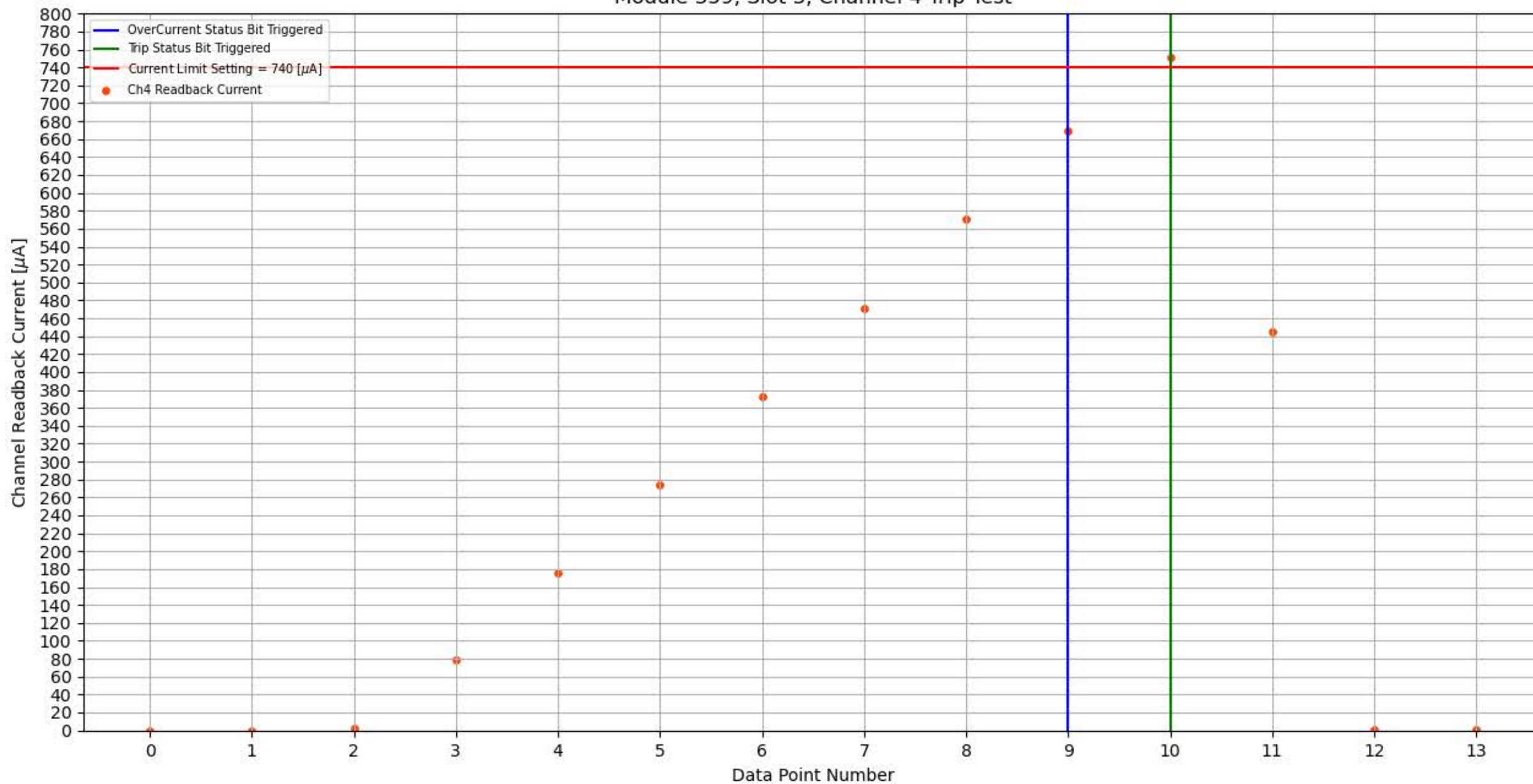
Module 359, Slot 3, Channel 4 Trip Test
