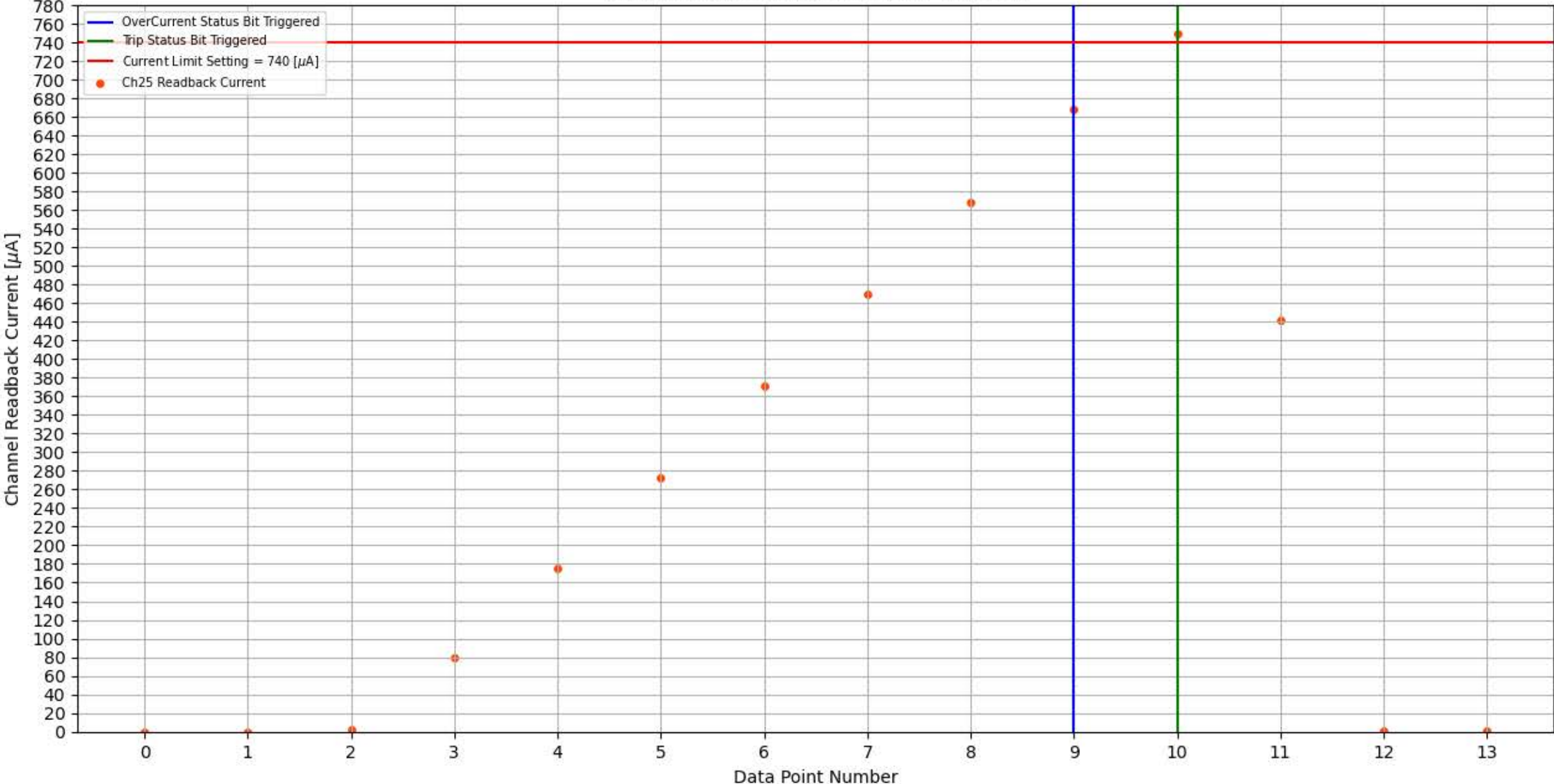
Module 359, Slot 3, Channel 25 Trip Test
