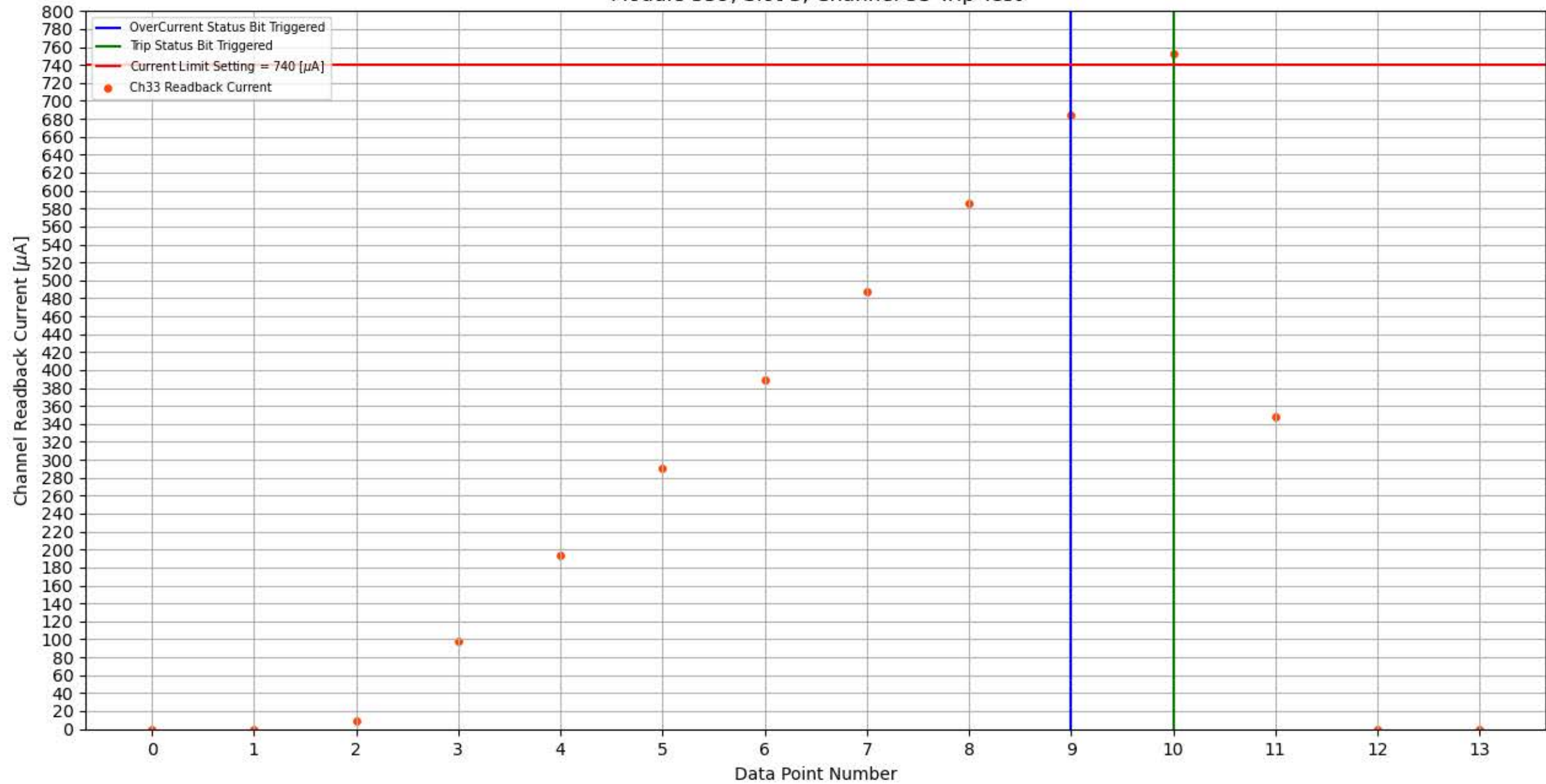
Module 359, Slot 3, Channel 33 Trip Test
