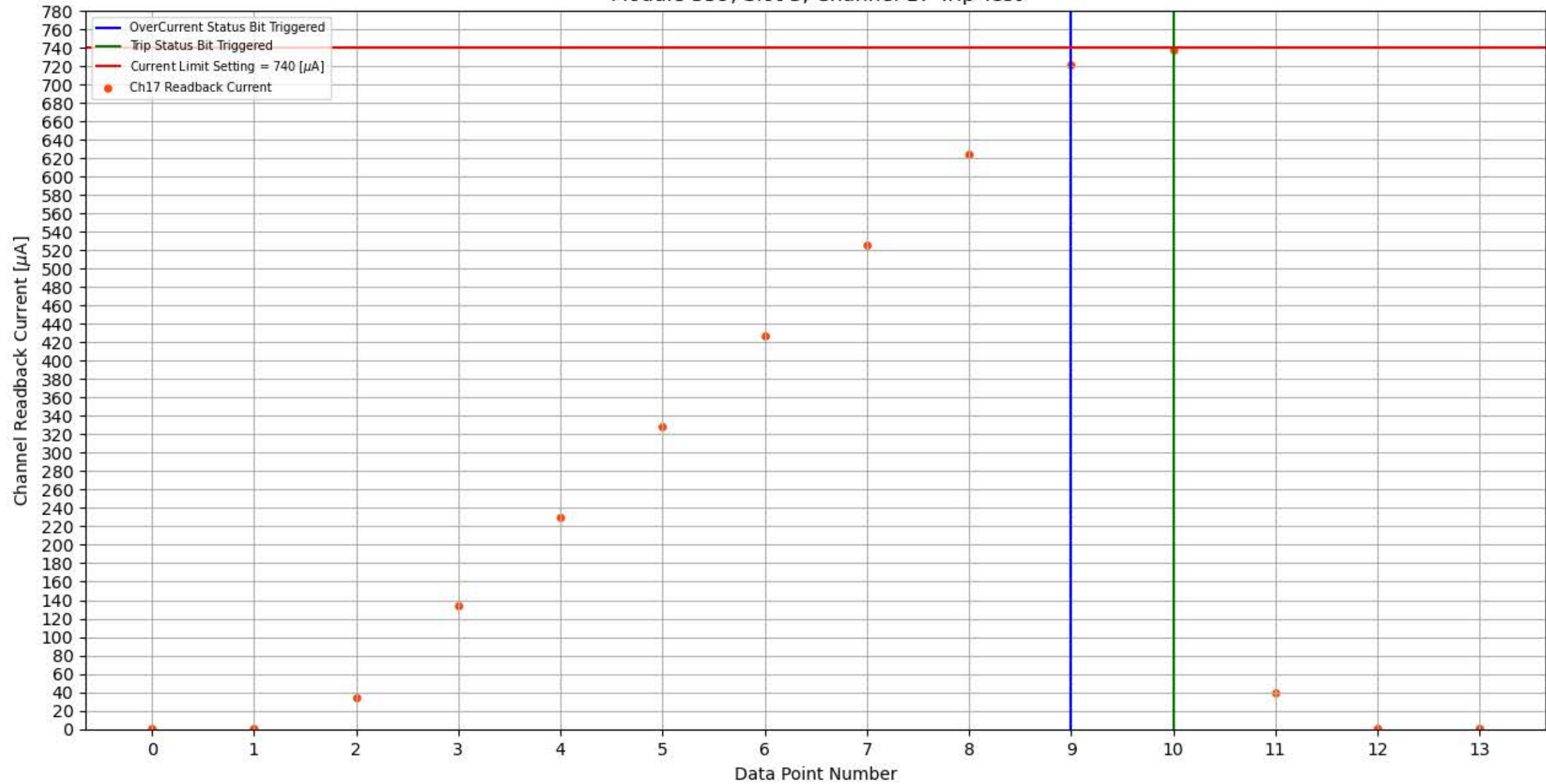
Module 359, Slot 3, Channel 17 Trip Test
