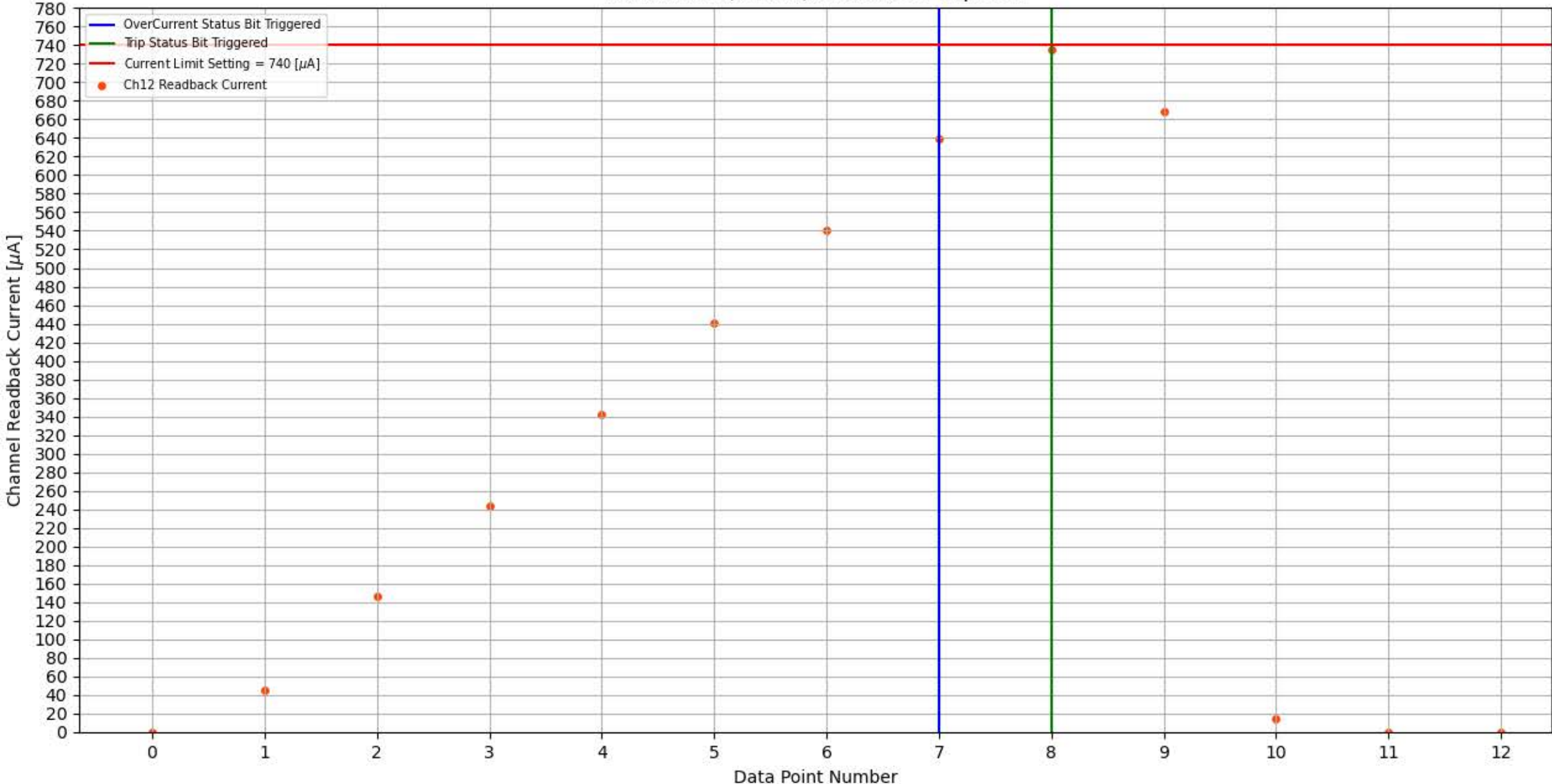
Module 359, Slot 3, Channel 12 Trip Test
