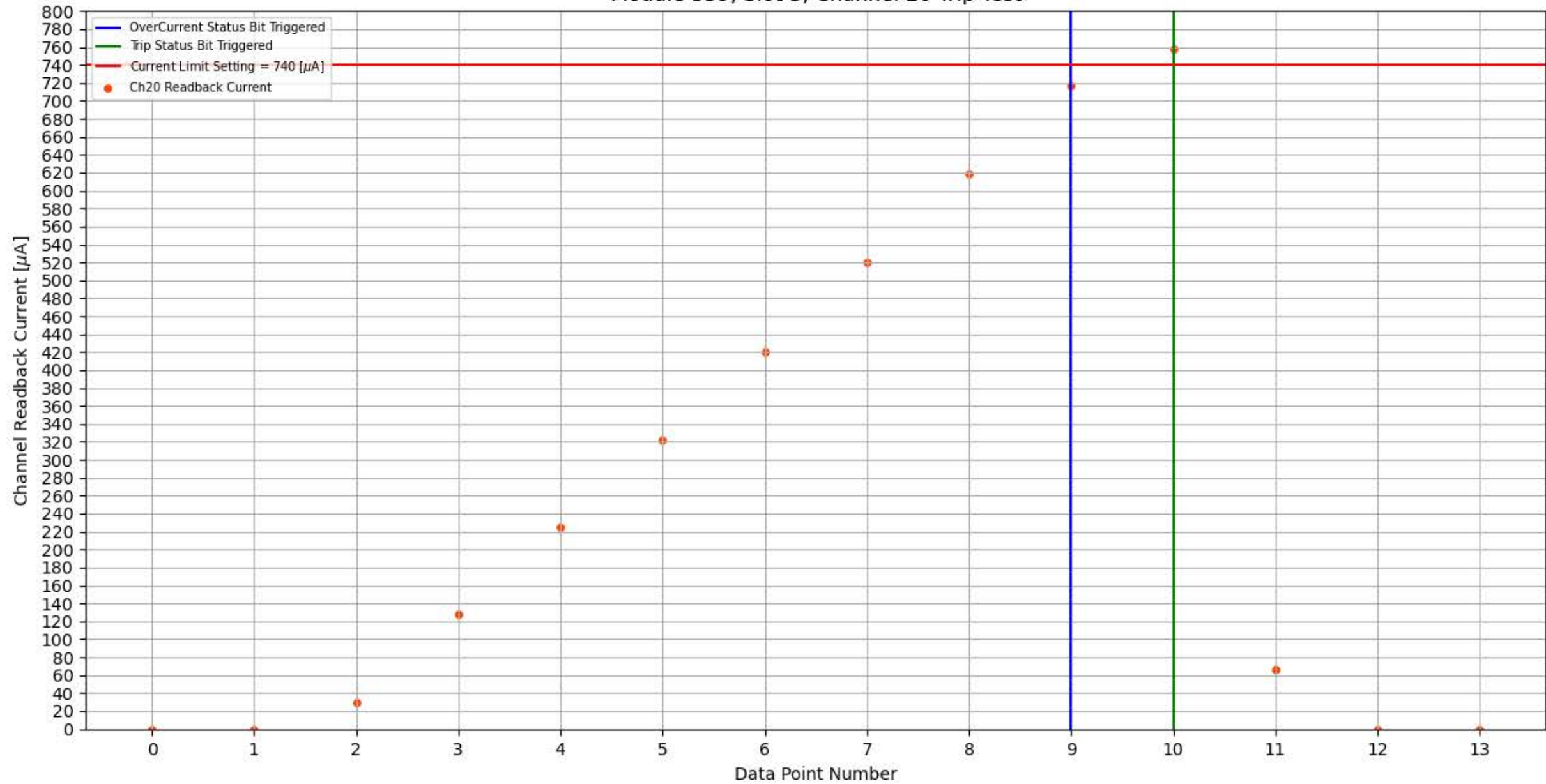
Module 359, Slot 3, Channel 20 Trip Test
