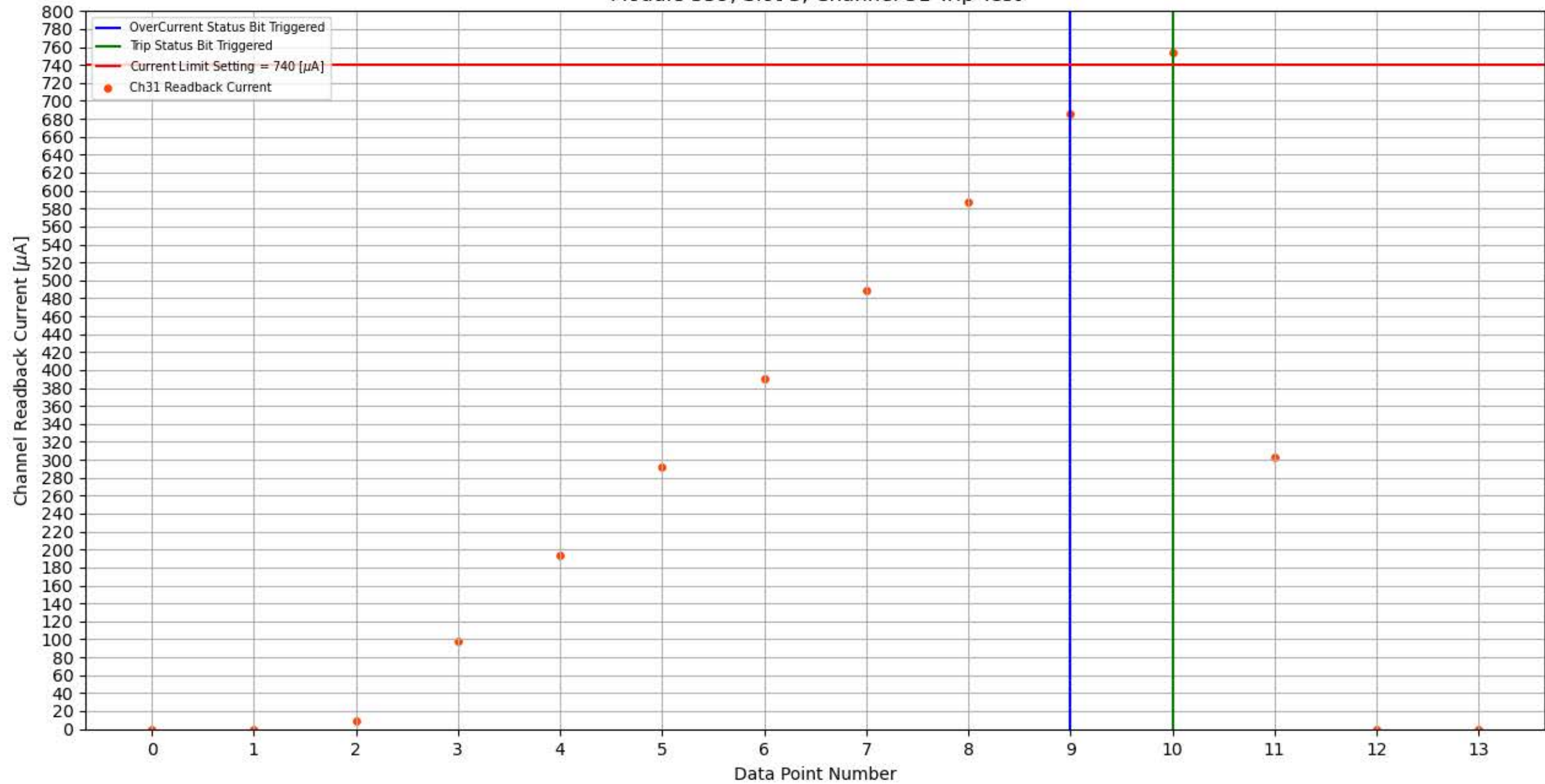
Module 359, Slot 3, Channel 31 Trip Test
