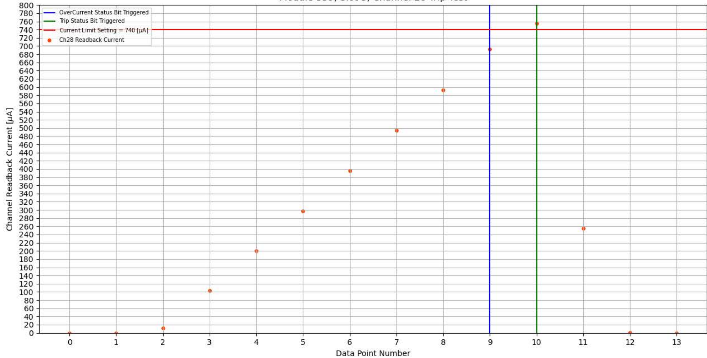
Module 359, Slot 3, Channel 28 Trip Test
