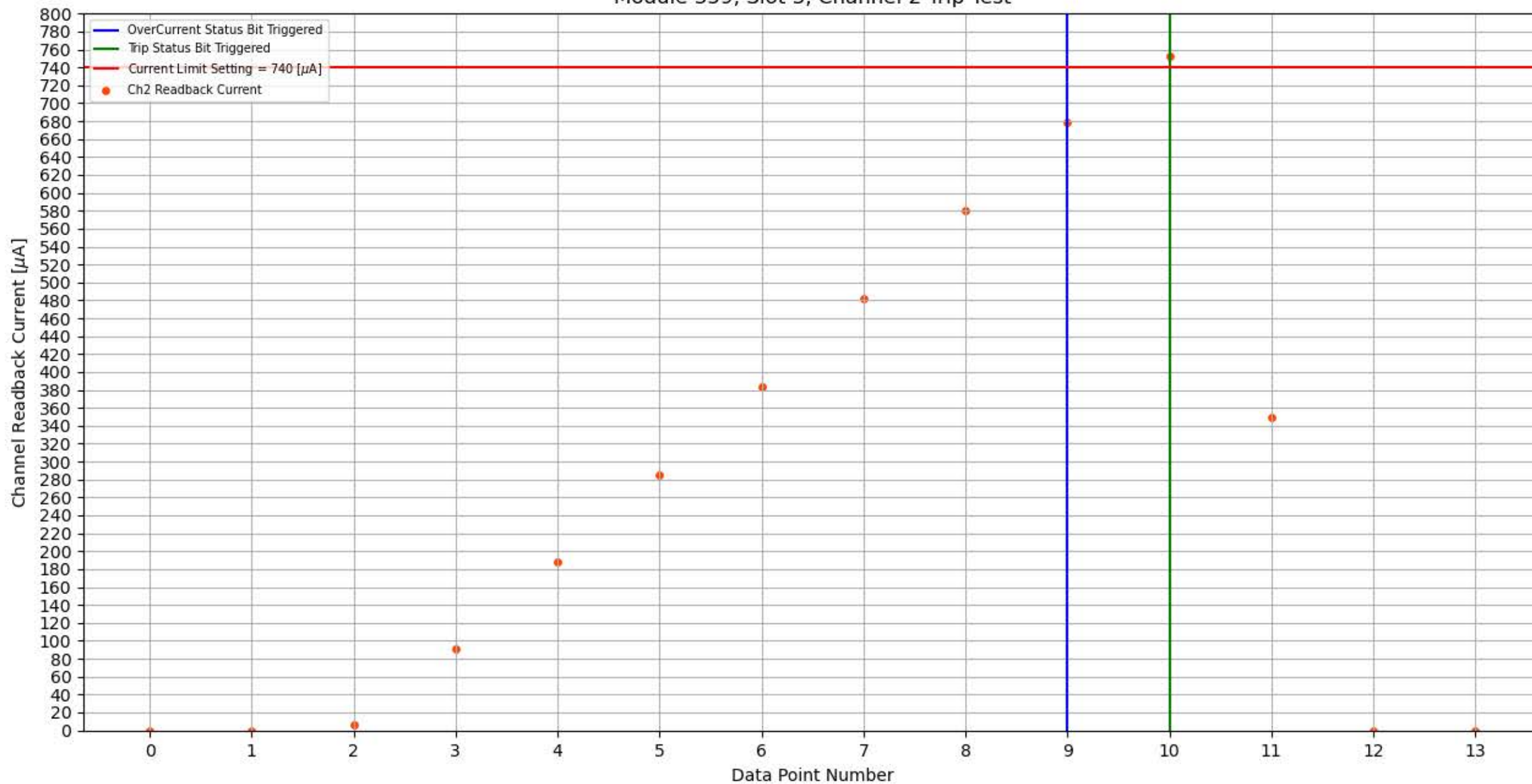
Module 359, Slot 3, Channel 2 Trip Test
