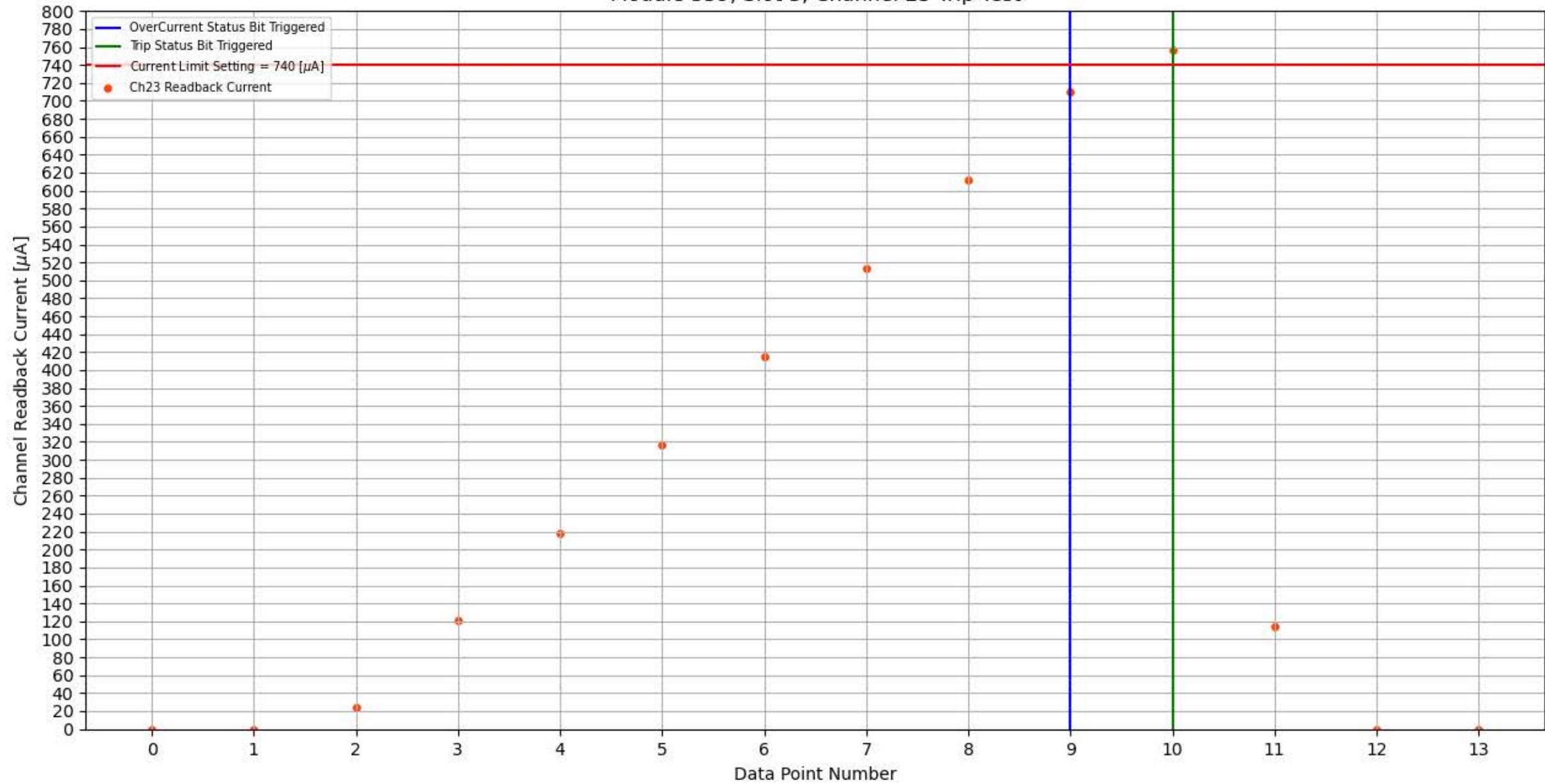
Module 359, Slot 3, Channel 23 Trip Test
