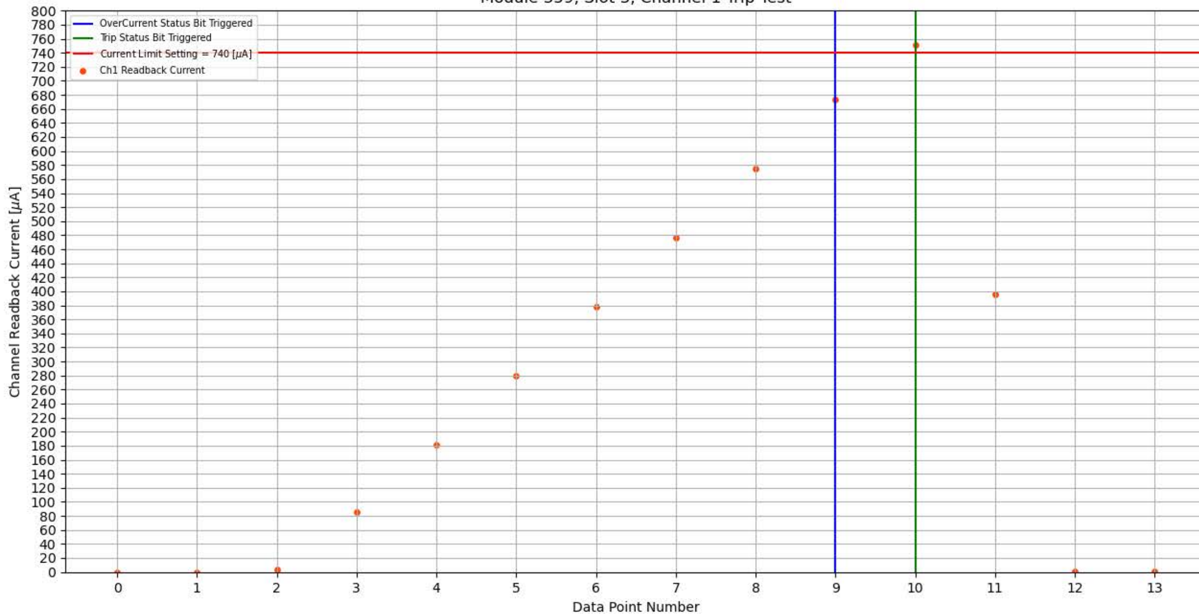
Module 359, Slot 3, Channel 1 Trip Test
