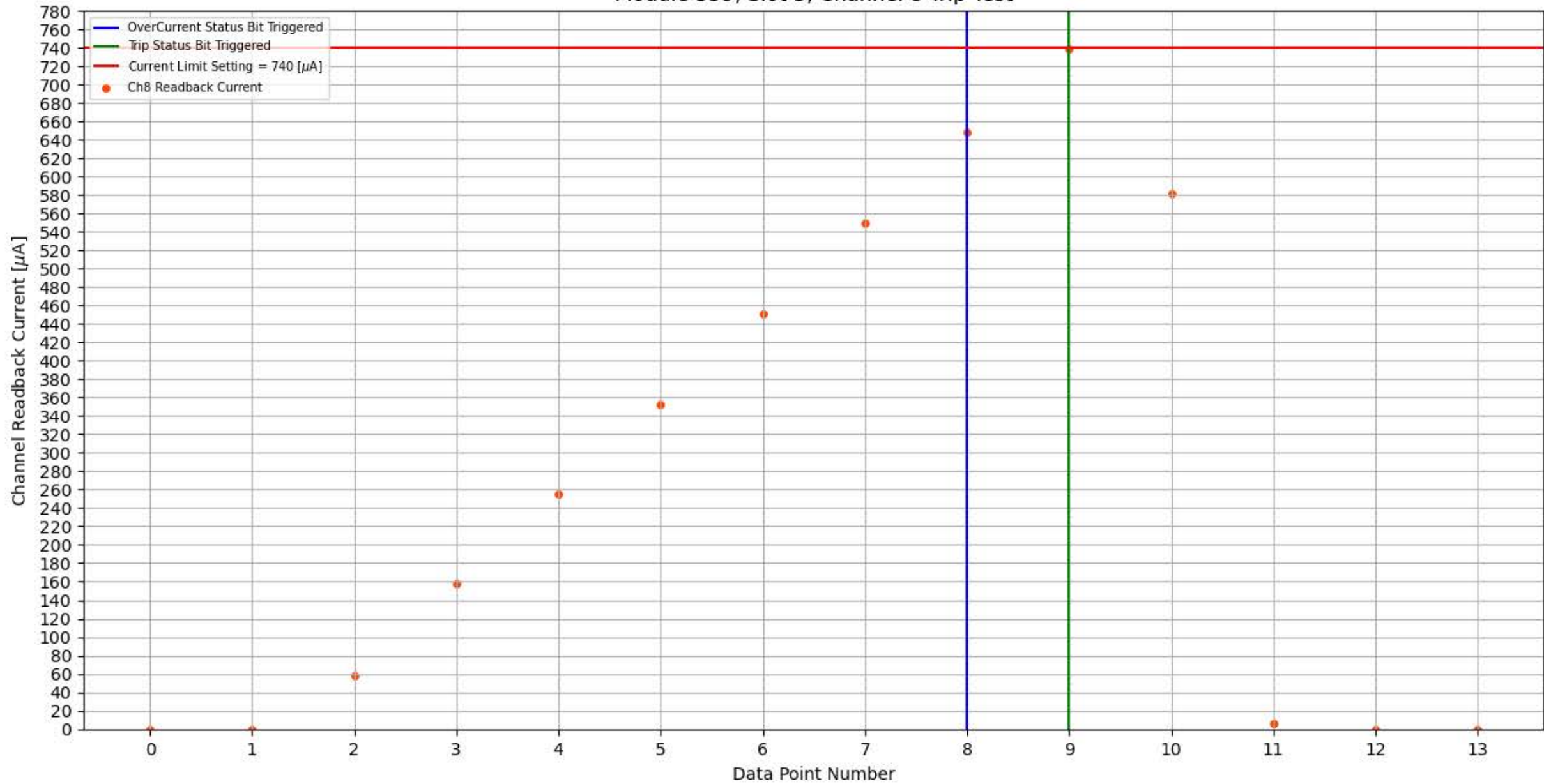
Module 359, Slot 3, Channel 8 Trip Test
