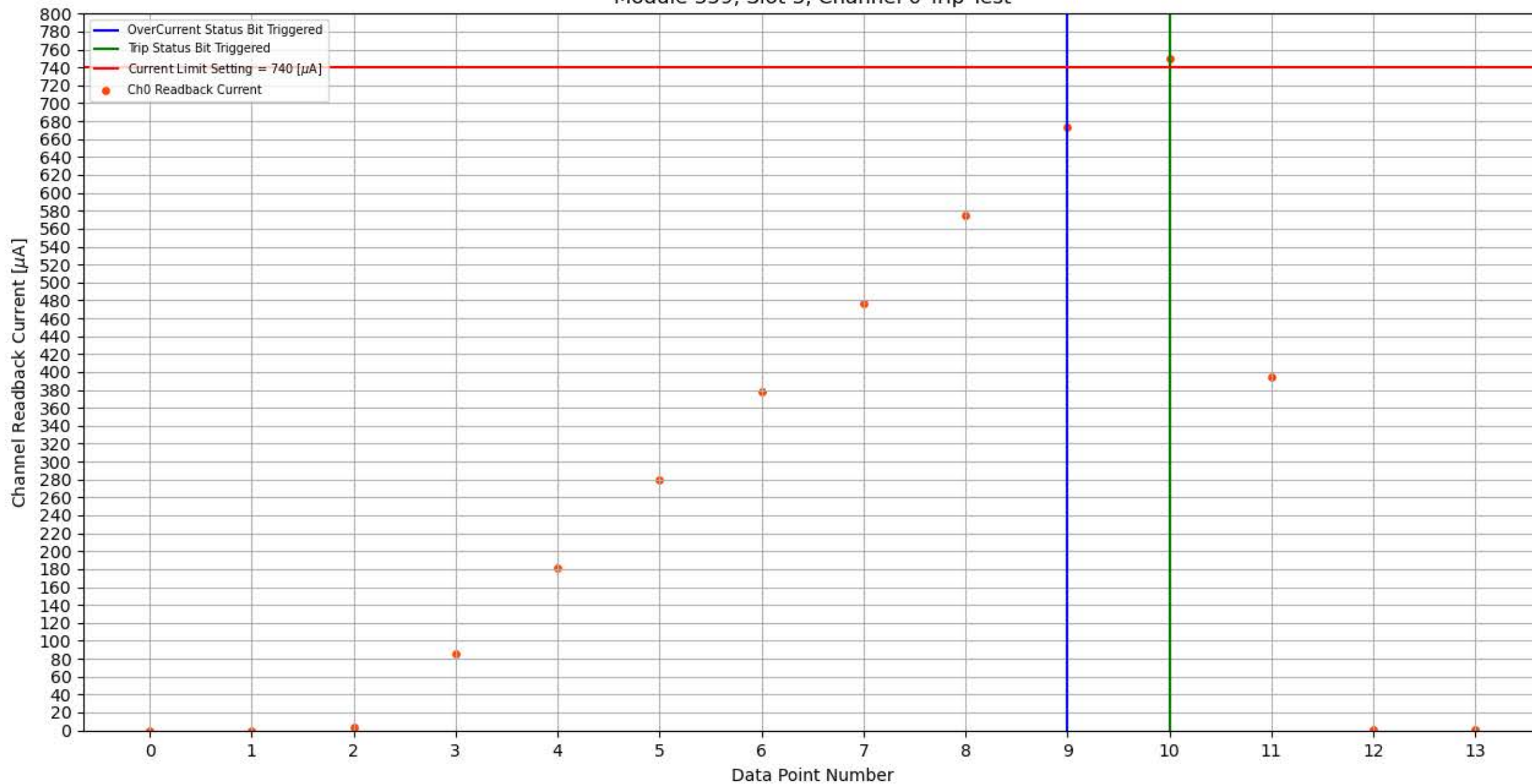
Module 359, Slot 3, Channel 0 Trip Test
