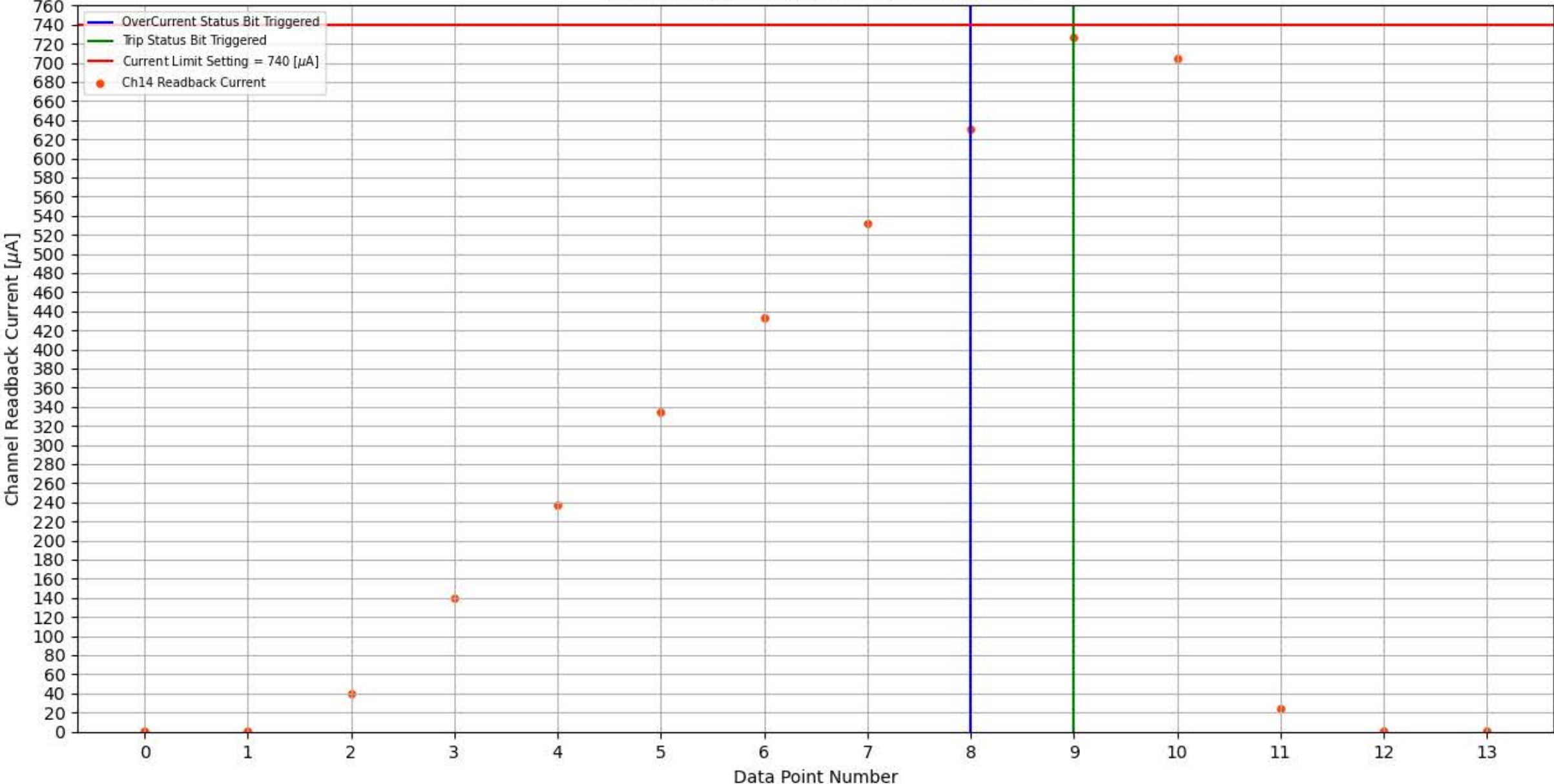
Module 359, Slot 3, Channel 14 Trip Test
