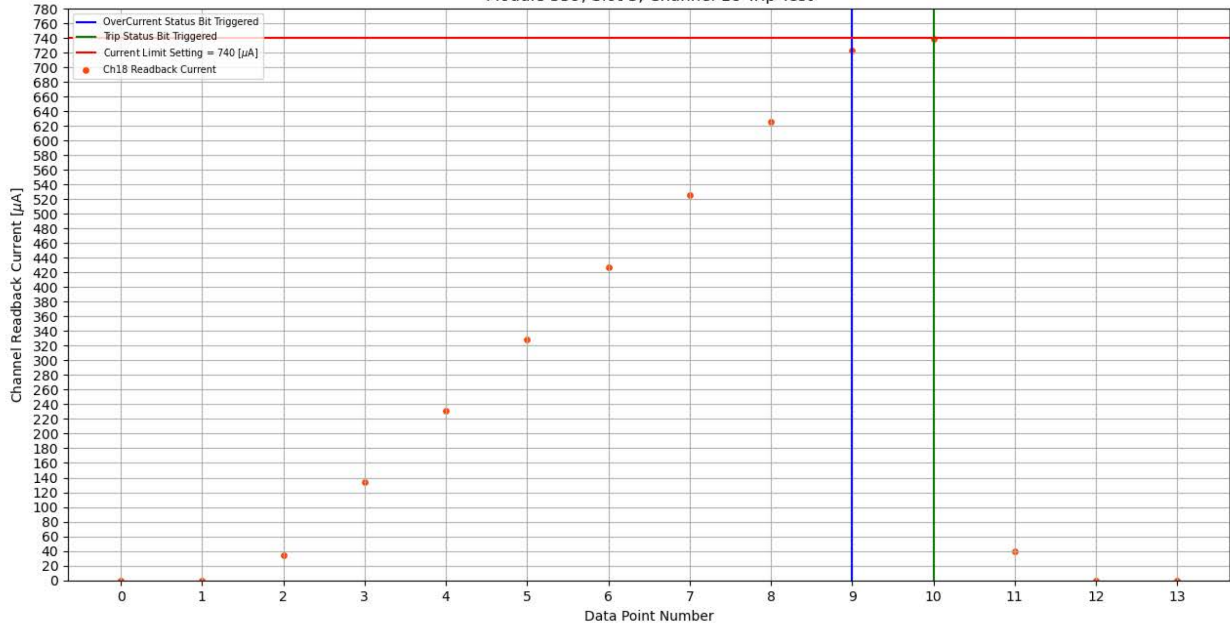
Module 359, Slot 3, Channel 18 Trip Test
