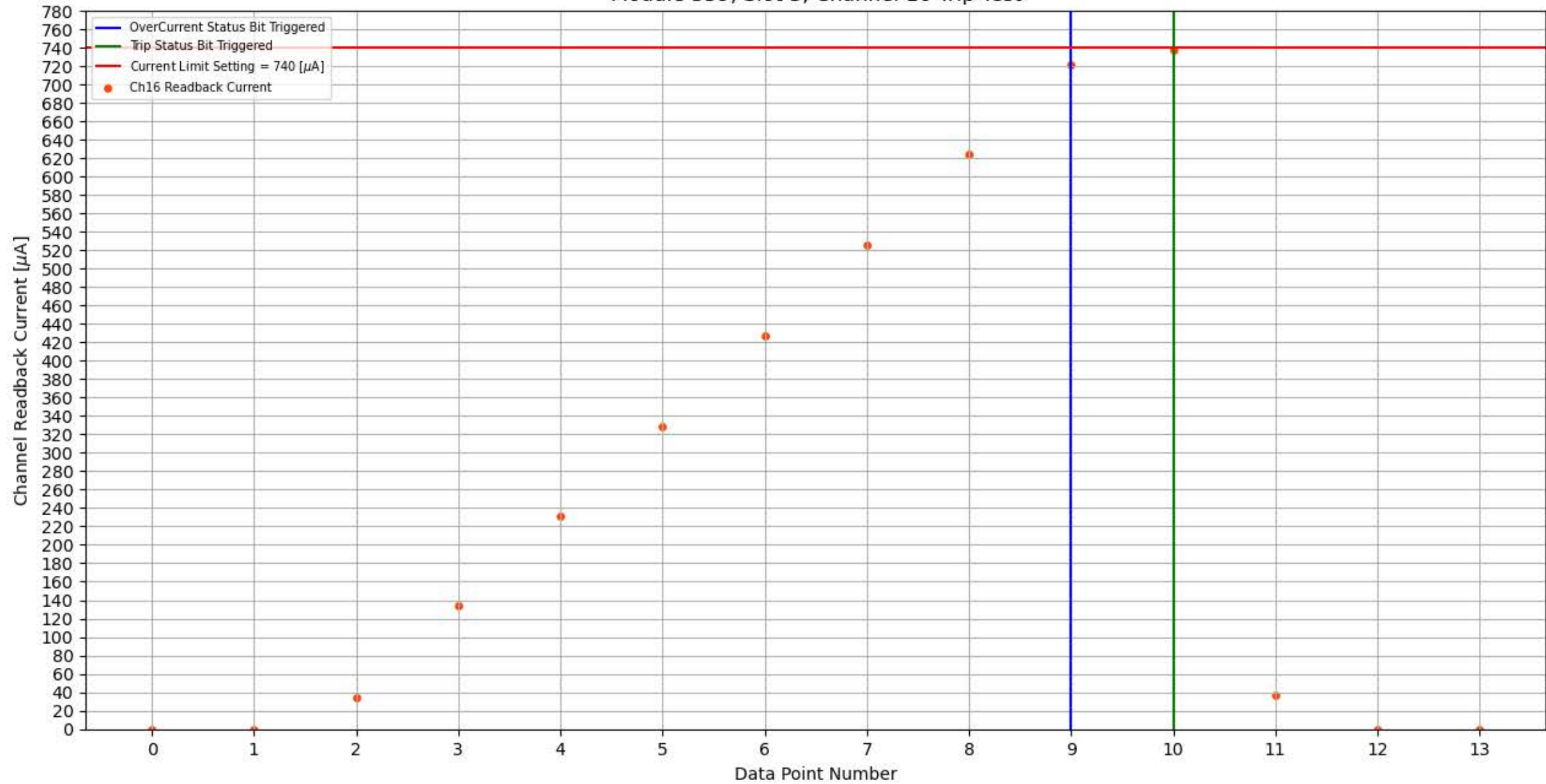
Module 359, Slot 3, Channel 16 Trip Test
