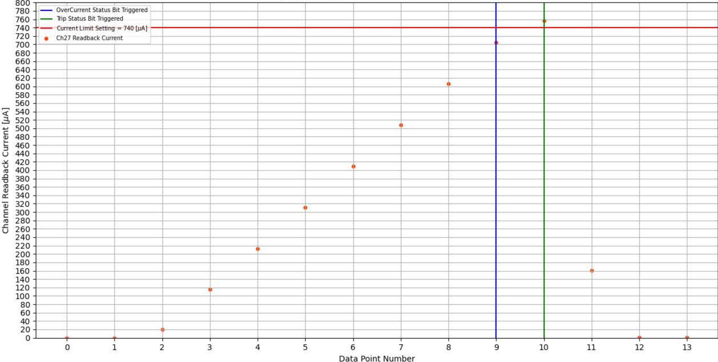
Module 359, Slot 3, Channel 27 Trip Test
