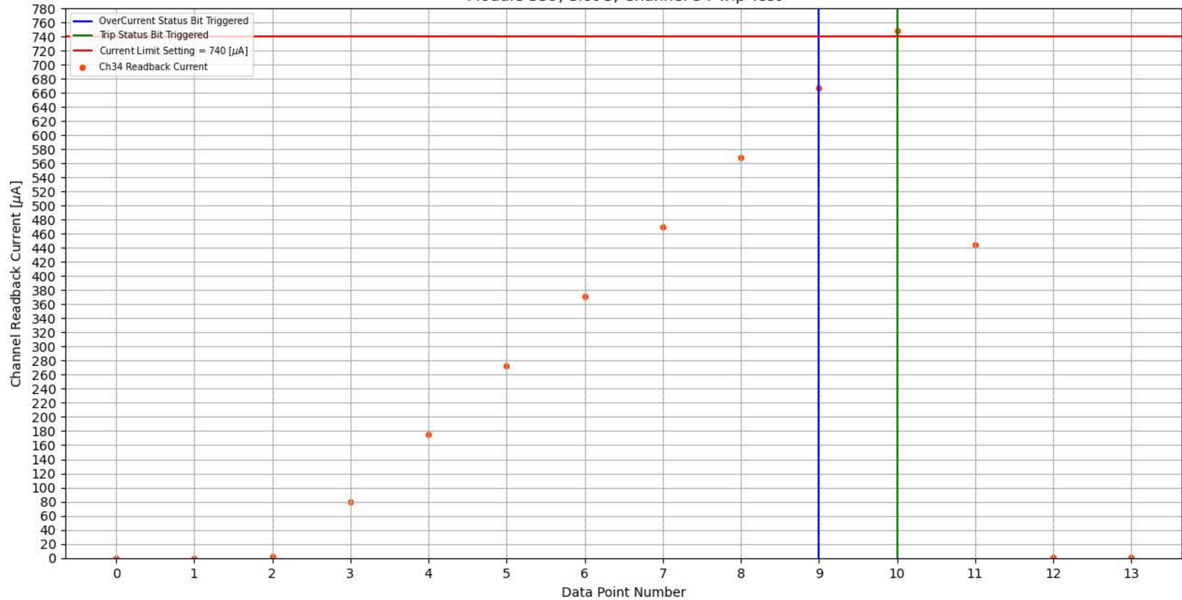
Module 359, Slot 3, Channel 34 Trip Test
