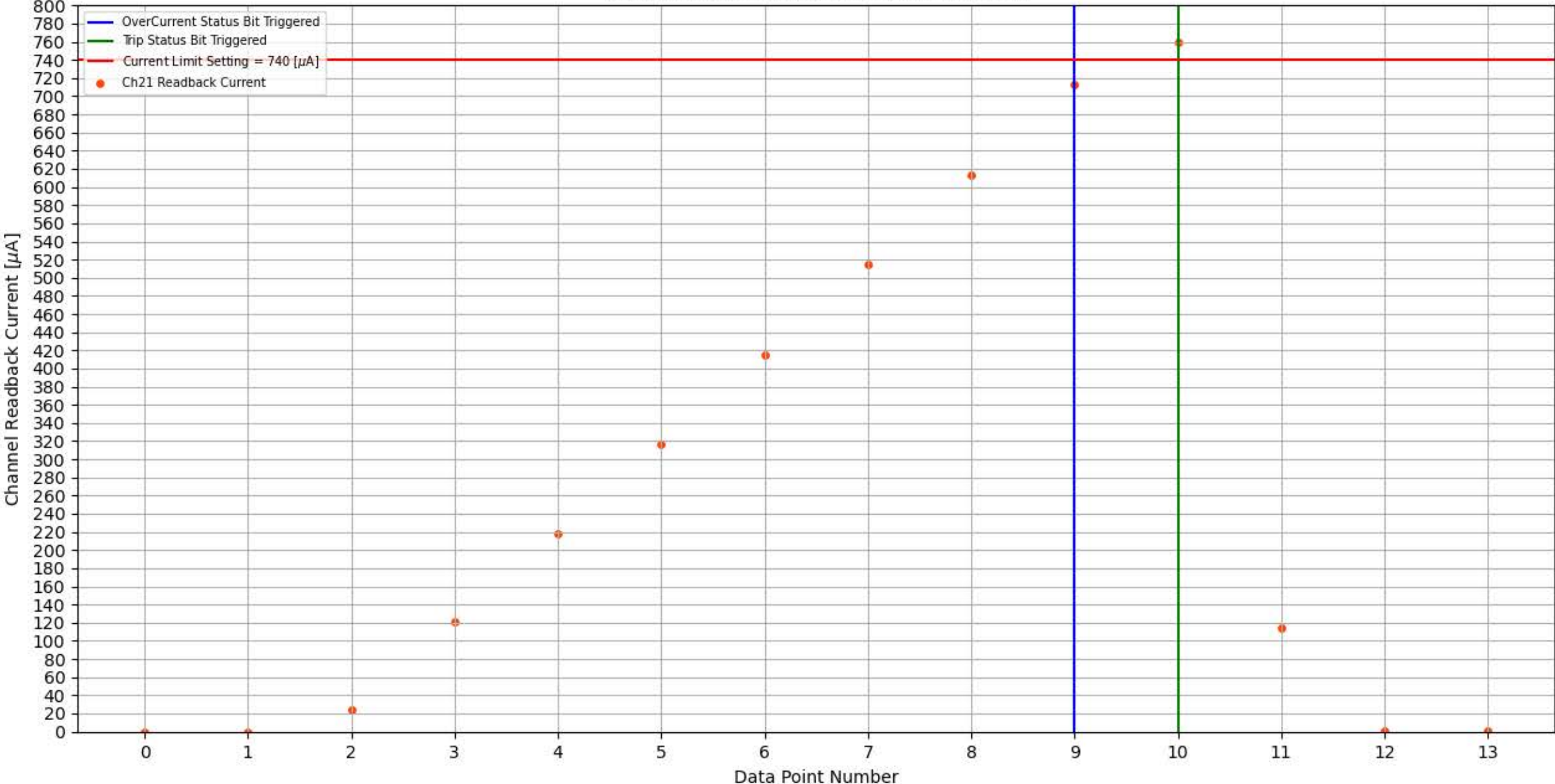
Module 359, Slot 3, Channel 21 Trip Test
