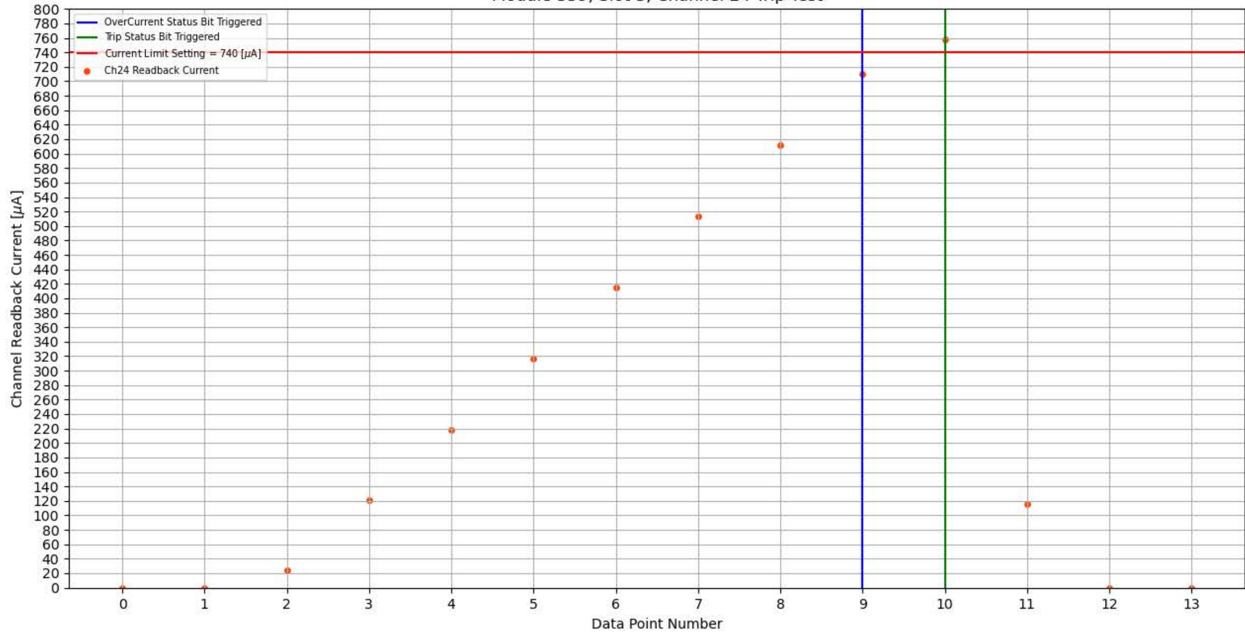
Module 359, Slot 3, Channel 24 Trip Test
