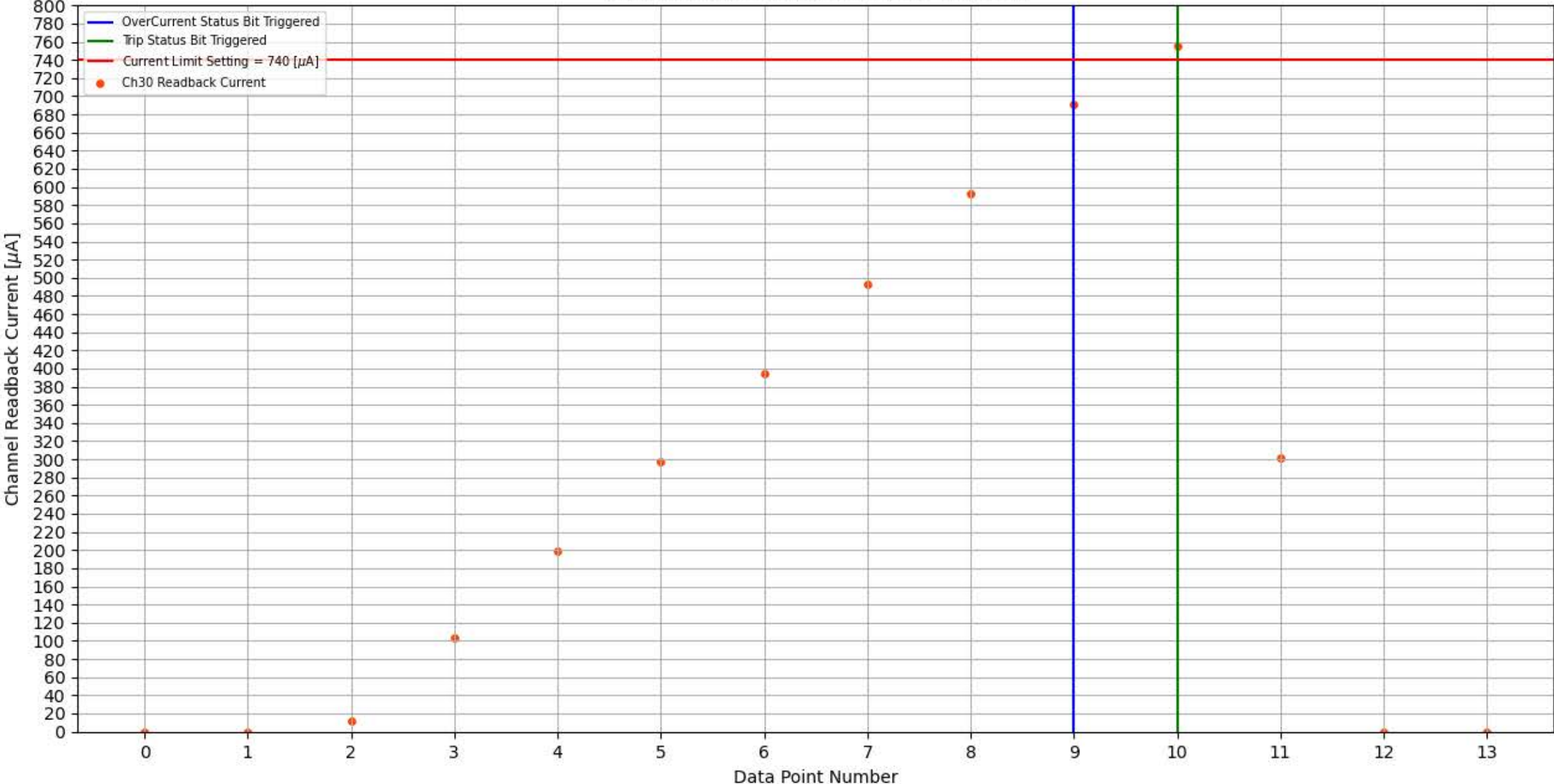
Module 359, Slot 3, Channel 30 Trip Test
