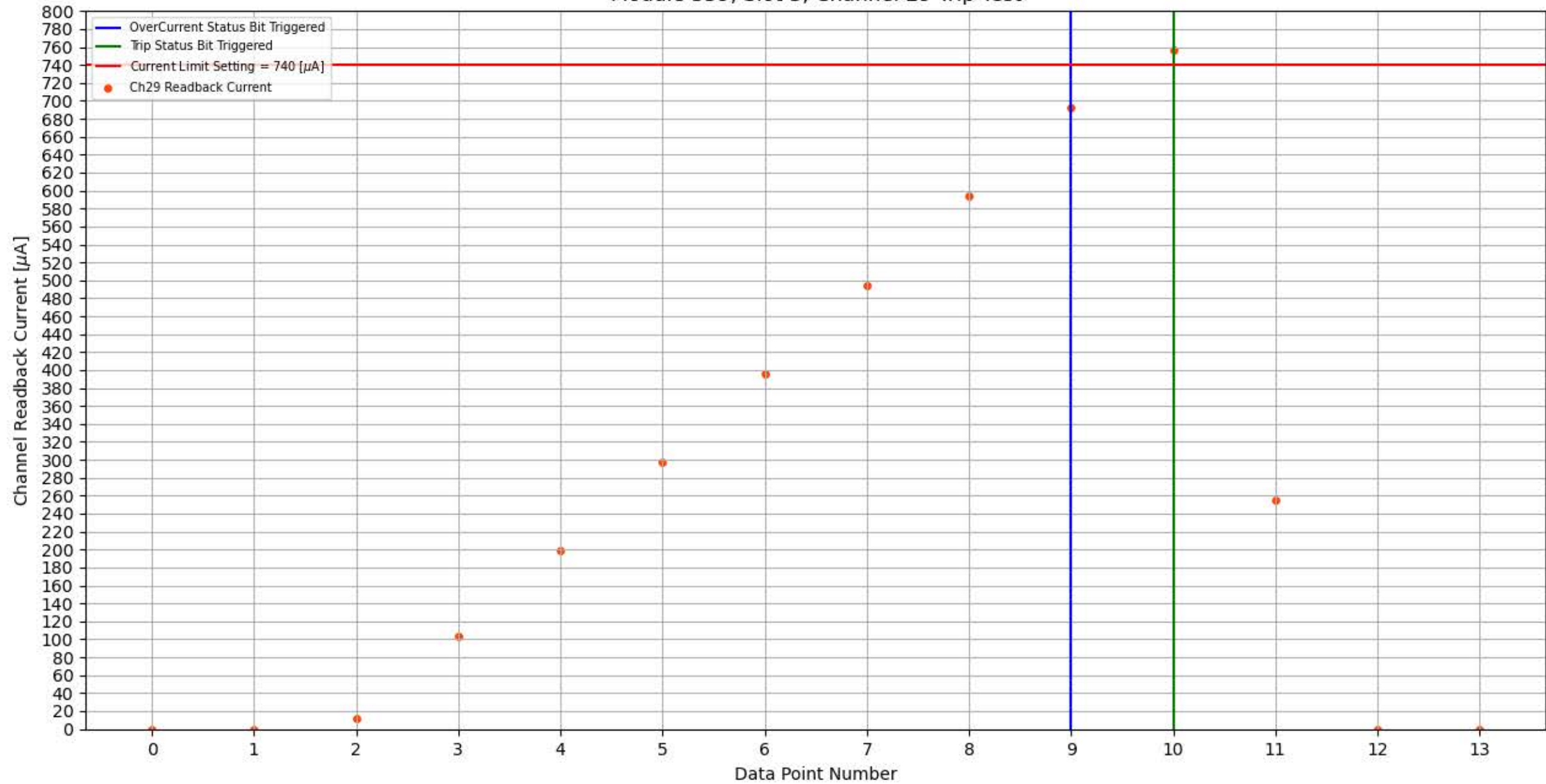
Module 359, Slot 3, Channel 29 Trip Test
