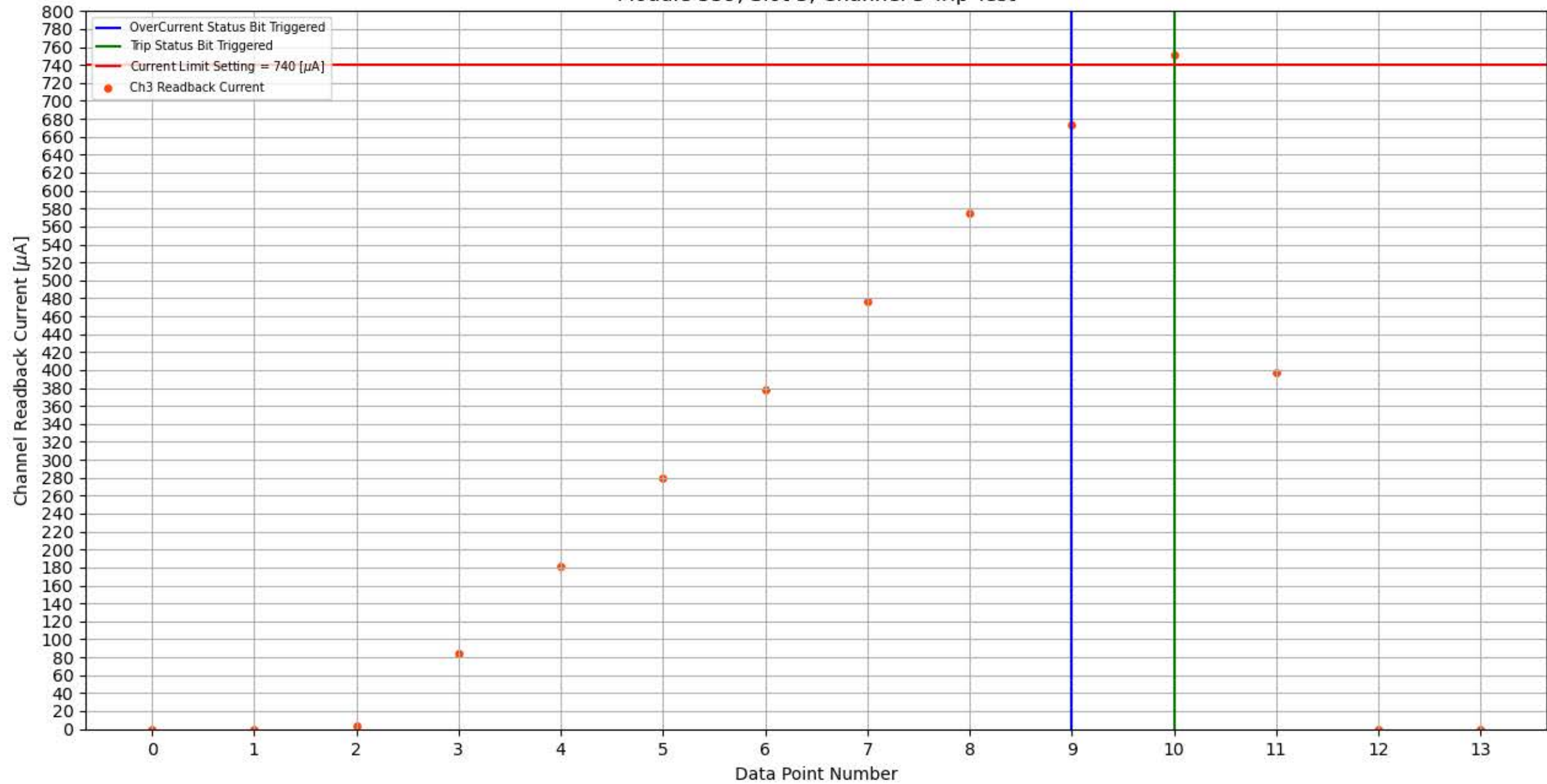
Module 359, Slot 3, Channel 3 Trip Test
