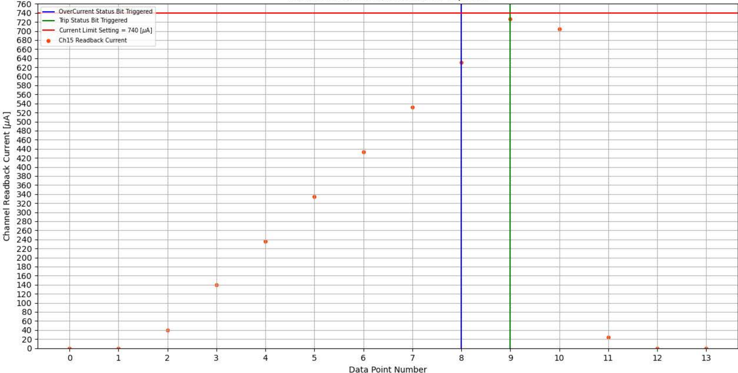
Module 359, Slot 3, Channel 15 Trip Test
