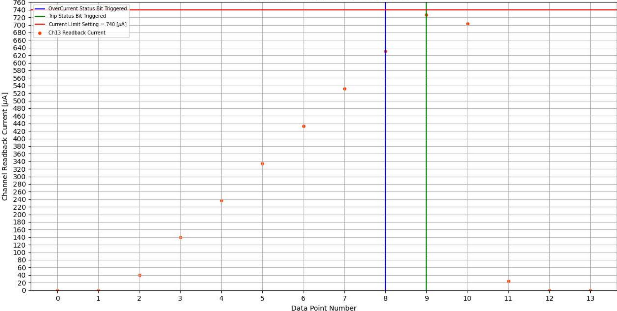
Module 359, Slot 3, Channel 13 Trip Test
