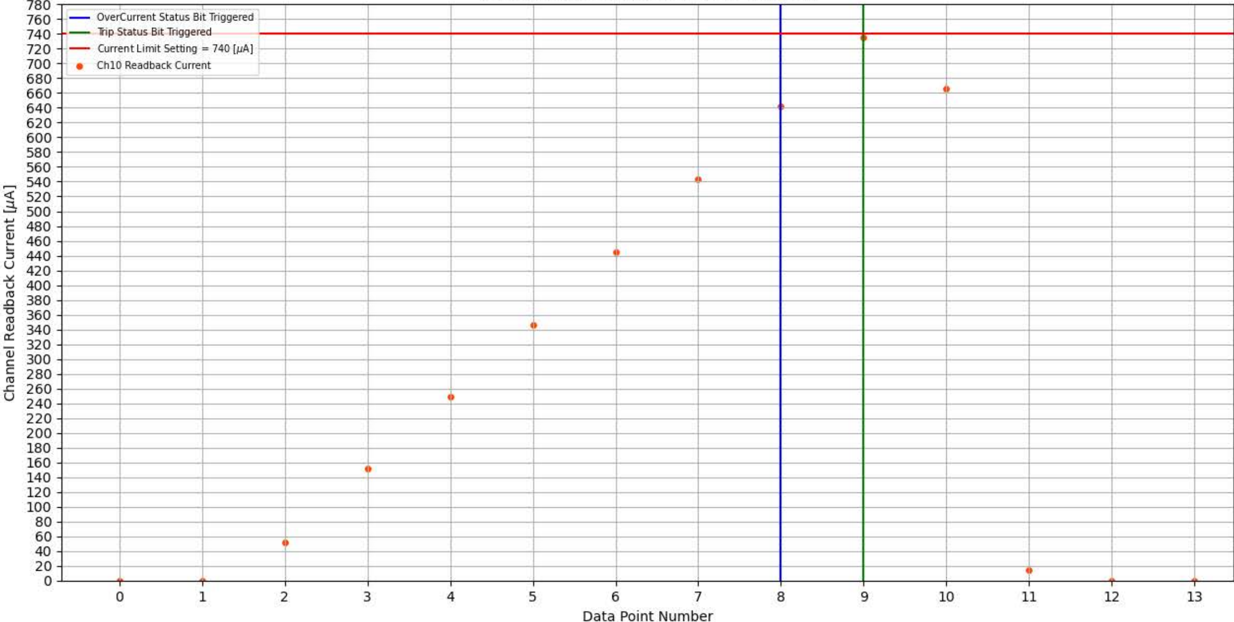
Module 359, Slot 3, Channel 10 Trip Test
