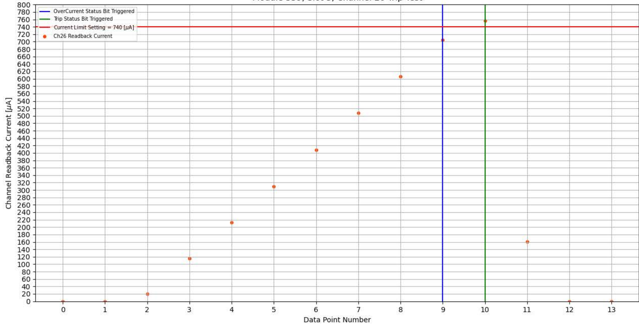
Module 359, Slot 3, Channel 26 Trip Test
