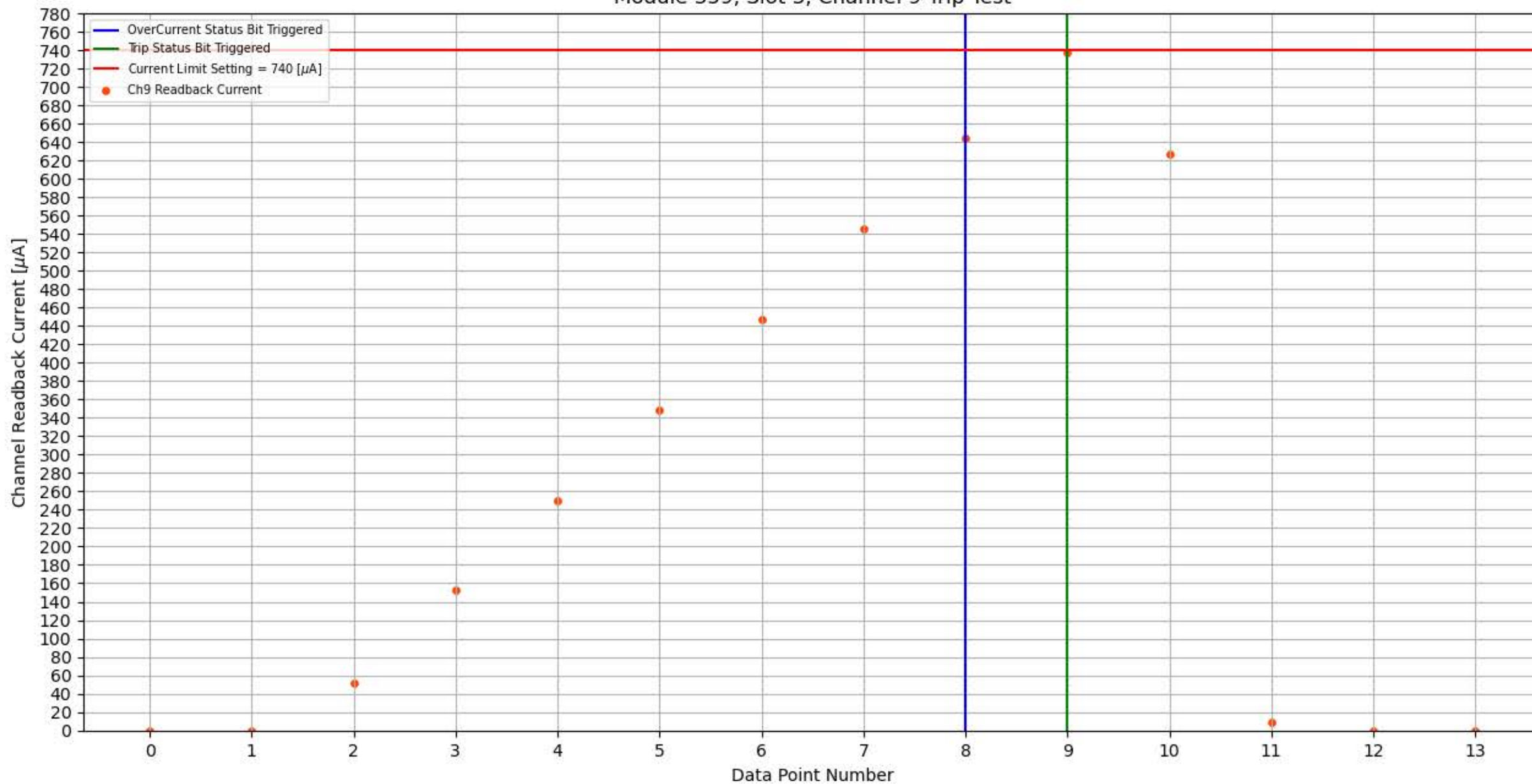
Module 359, Slot 3, Channel 9 Trip Test
