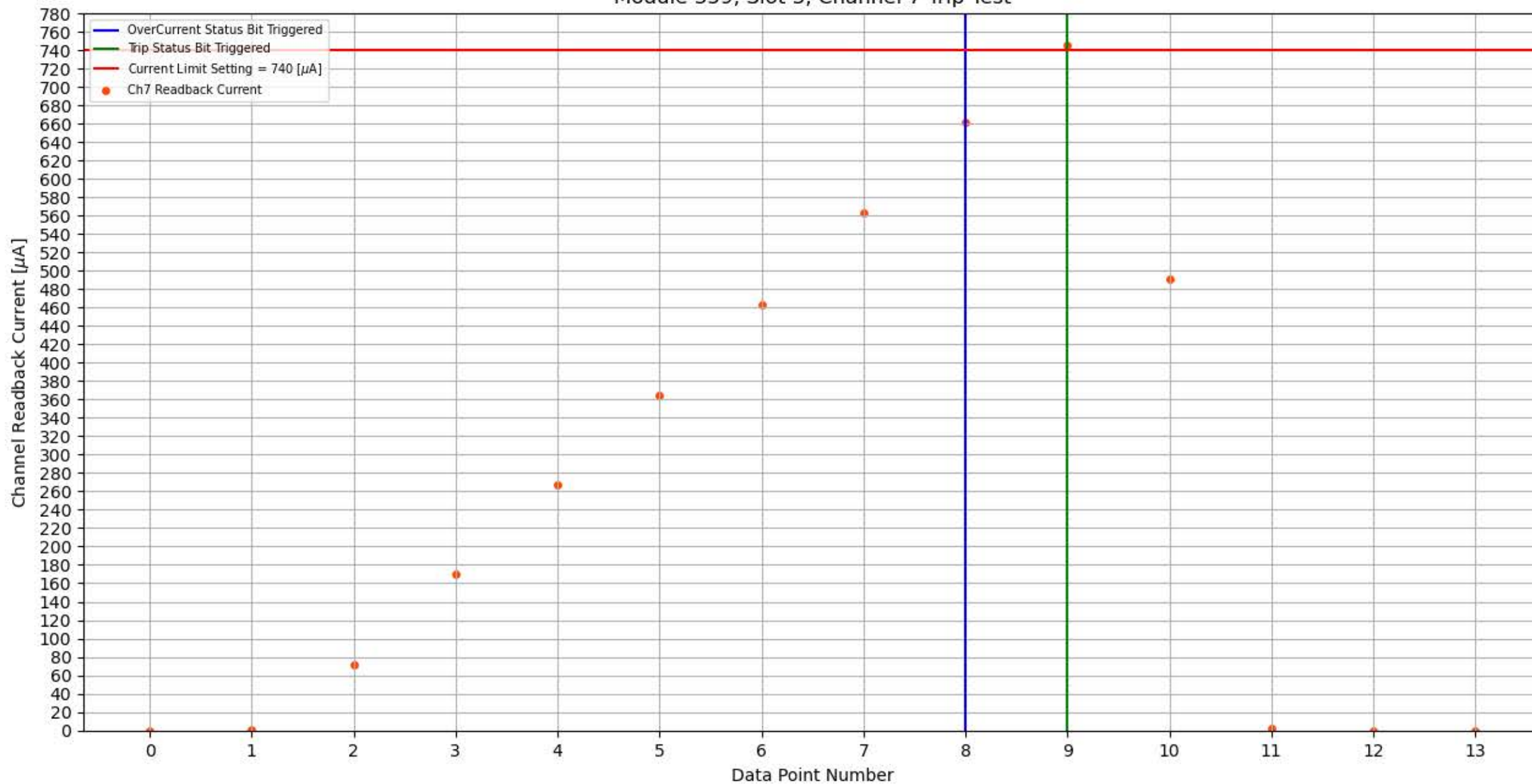
Module 359, Slot 3, Channel 7 Trip Test
