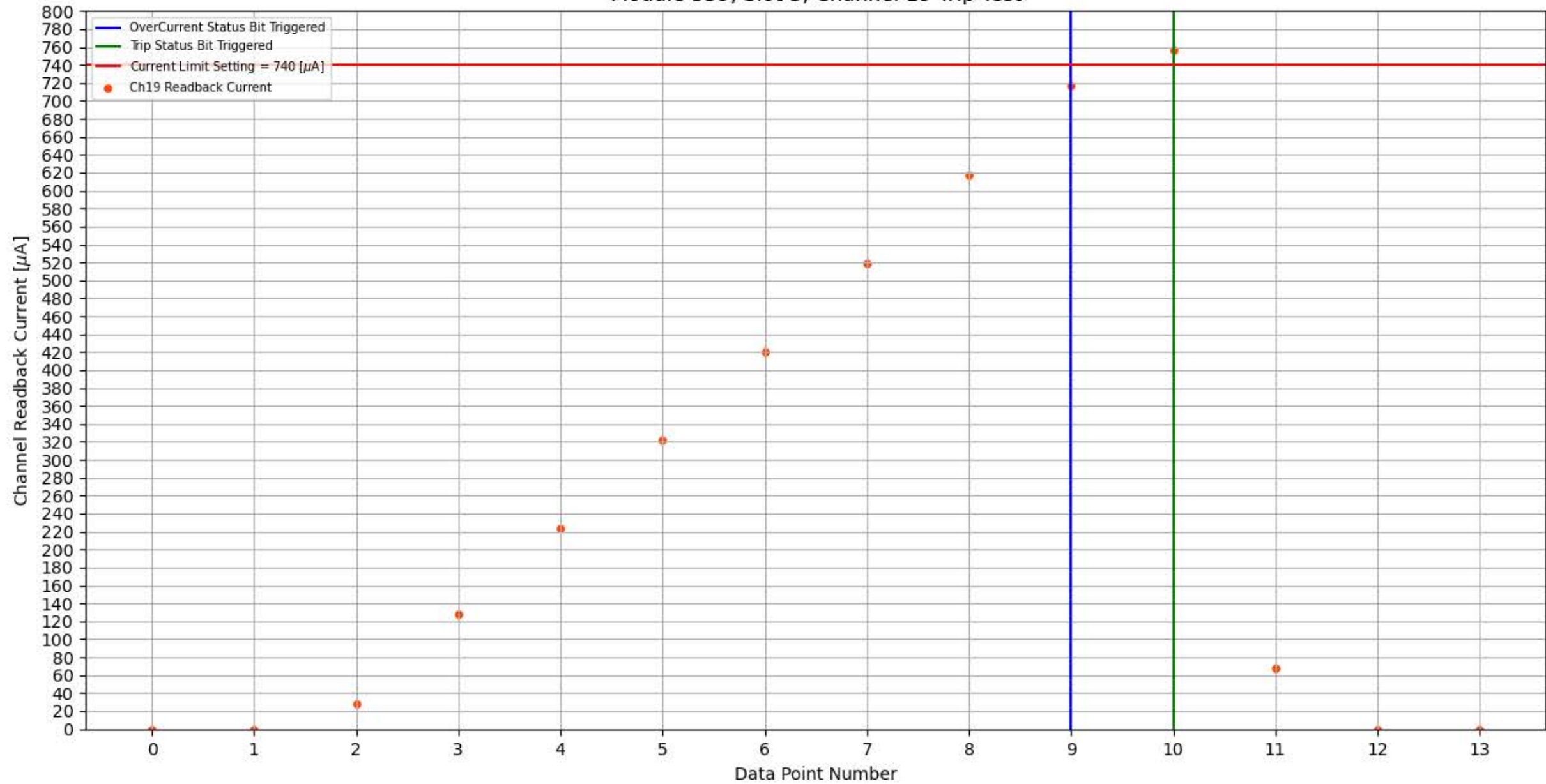
Module 359, Slot 3, Channel 19 Trip Test
