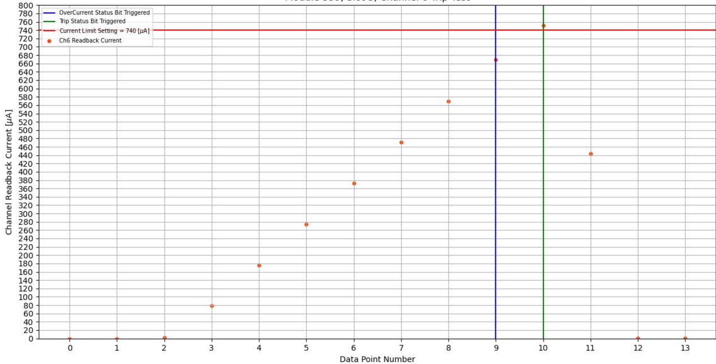
Module 359, Slot 3, Channel 6 Trip Test
