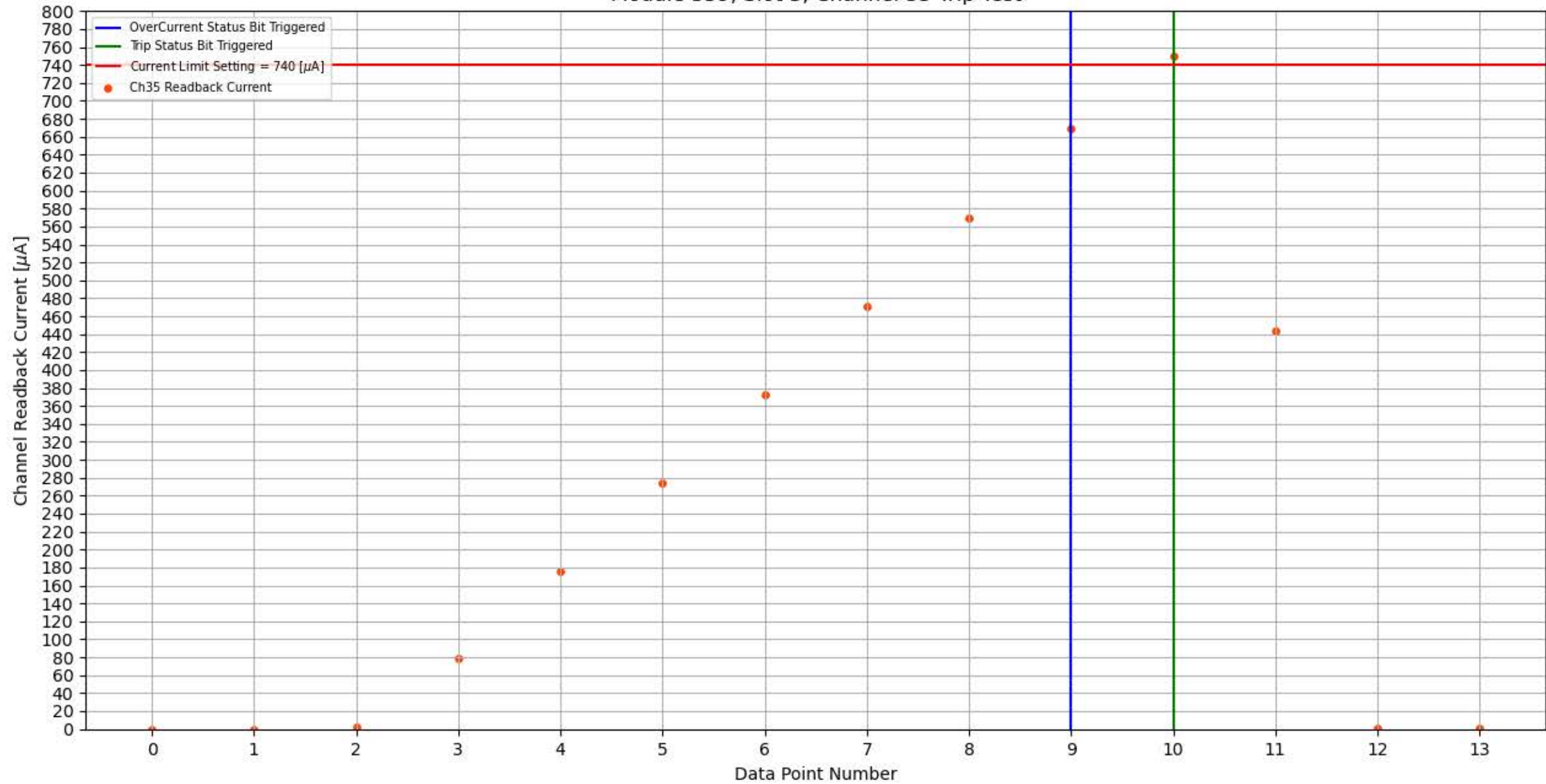
Module 359, Slot 3, Channel 35 Trip Test
