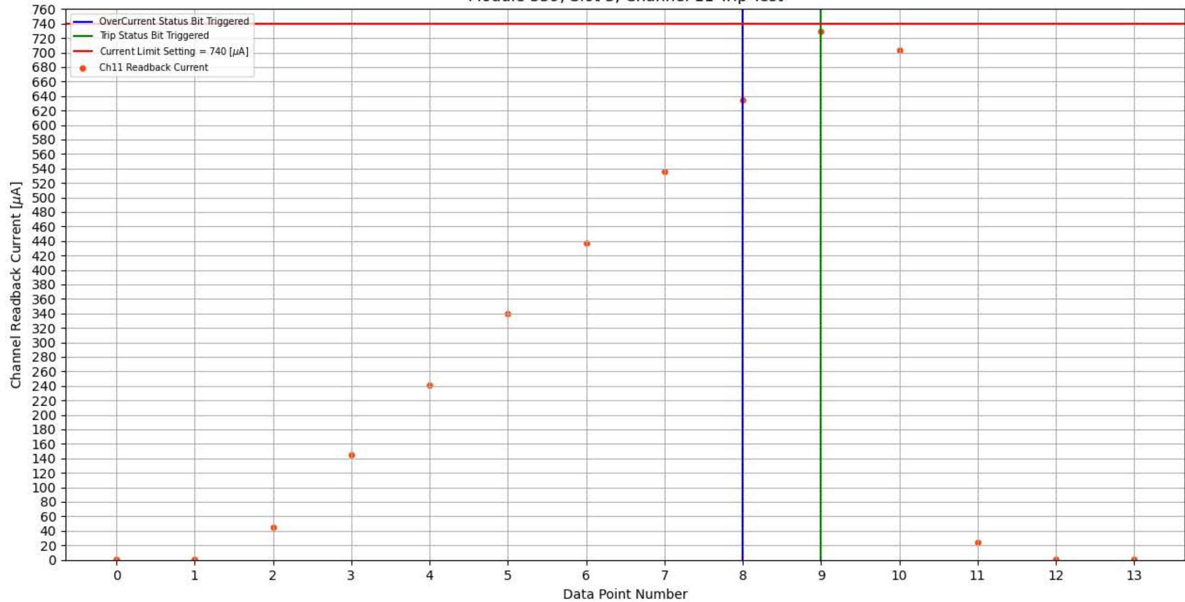
Module 359, Slot 3, Channel 11 Trip Test
