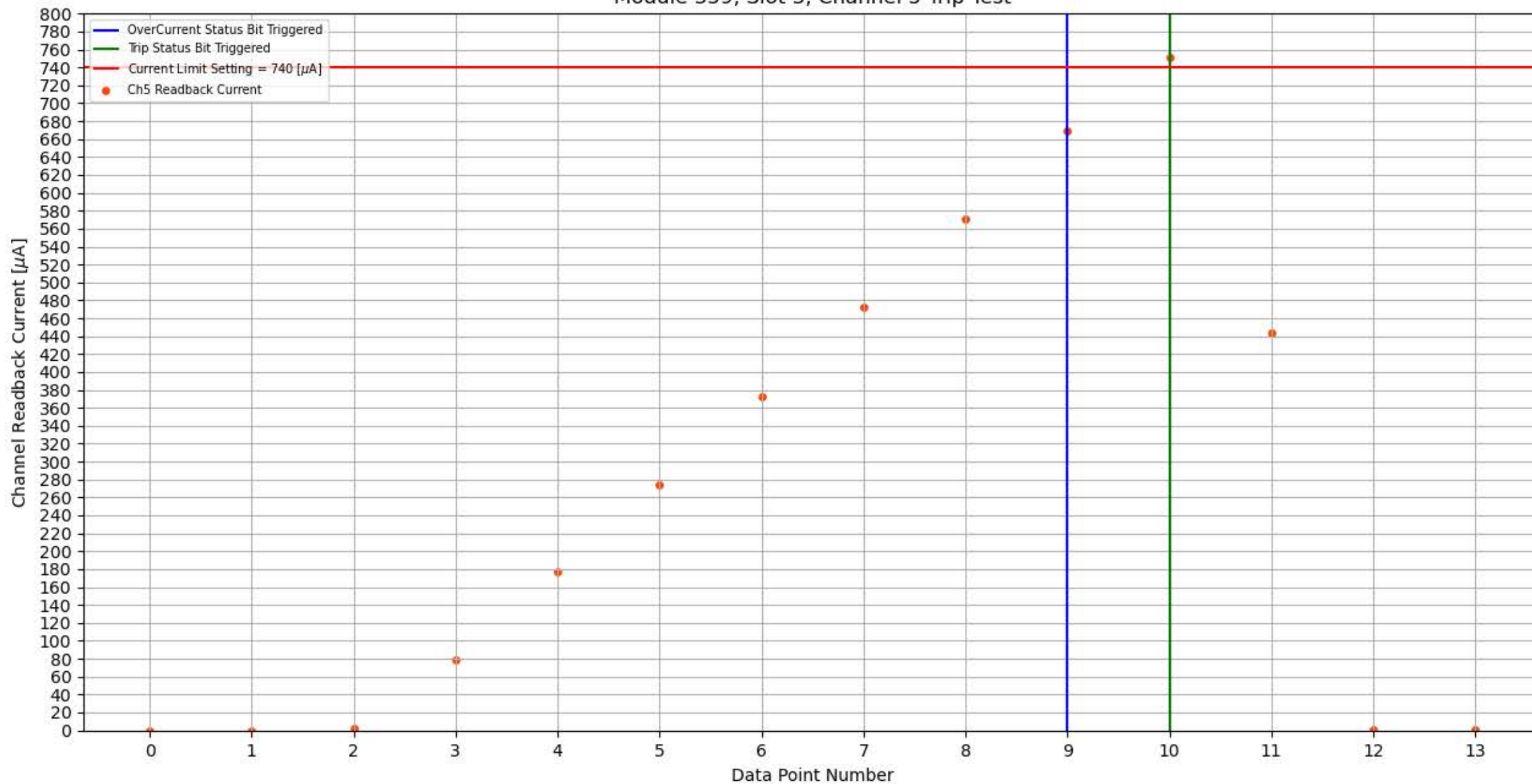
Module 359, Slot 3, Channel 5 Trip Test
